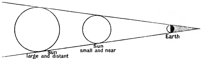
Fig. 37. Earth's Shadow.
